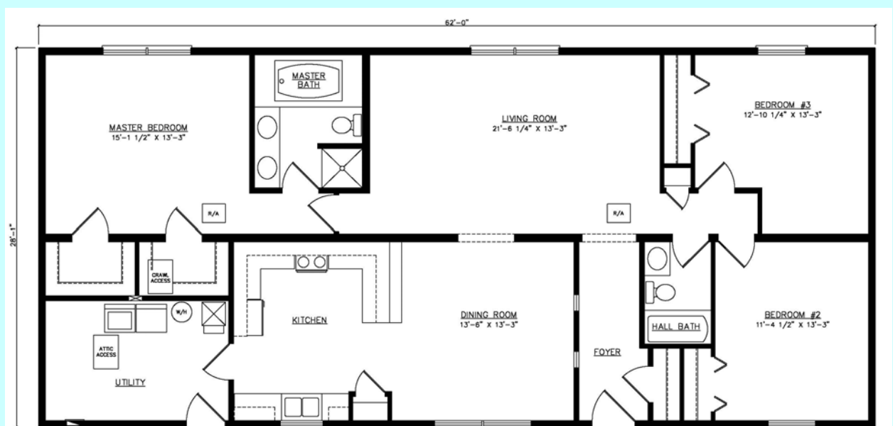
Crawlspace Plan
