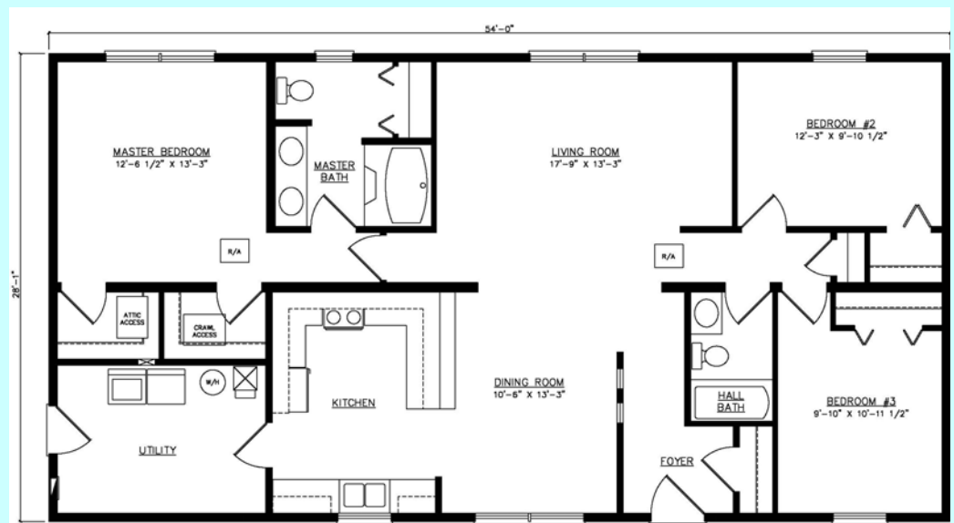
Crawlspace Plan
