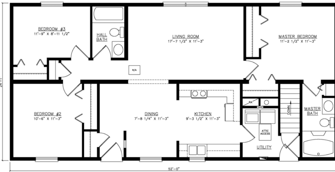
Federal I Basement Plan
