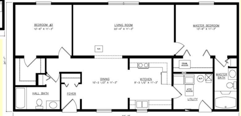
Federal III Crawlspace Plan
