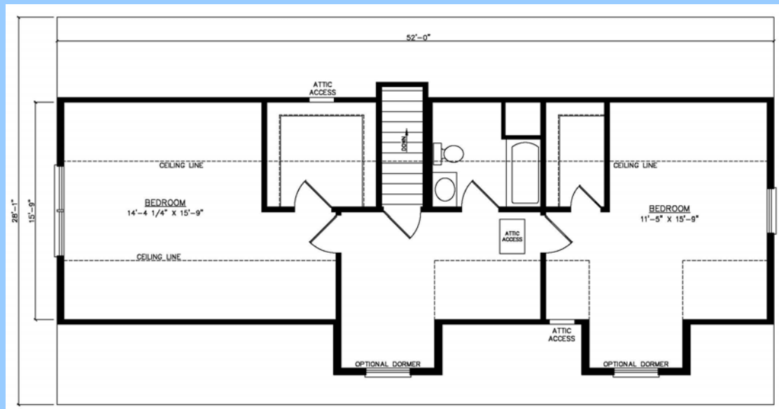
Proposed Upstairs Layout
